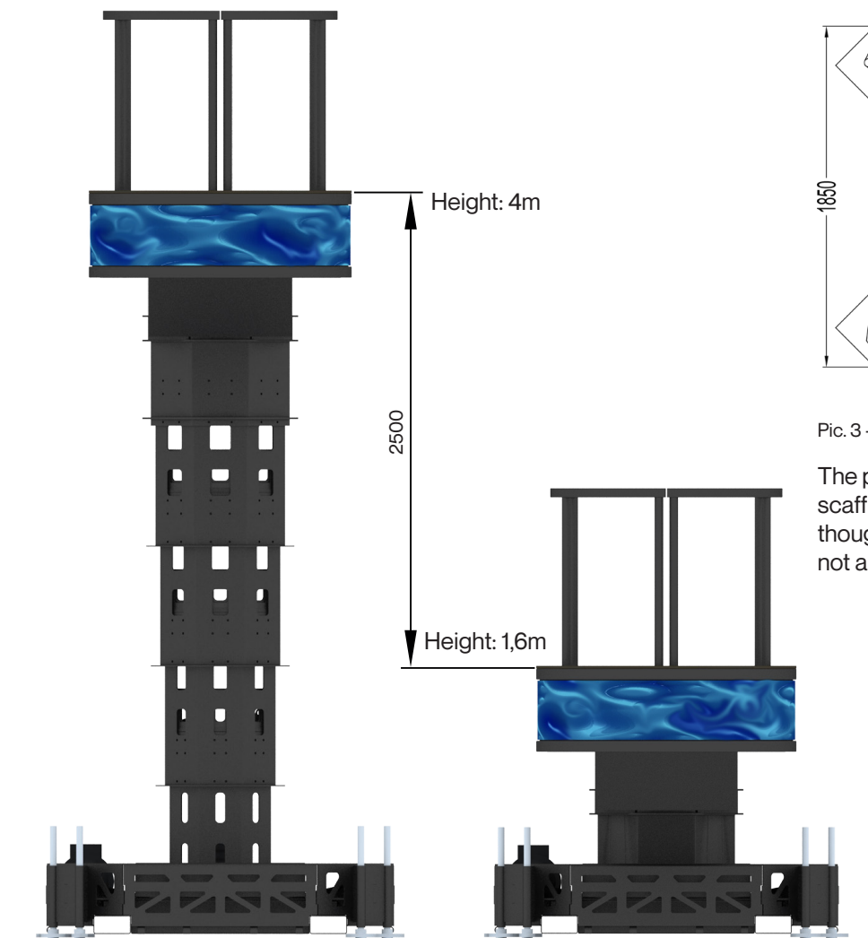
Pic. 4 - Drawing, base
