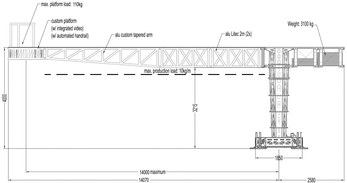
Pic. 2 - Drawing, side
