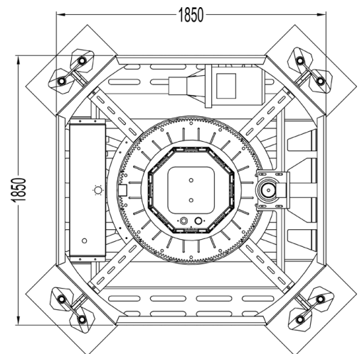
Pic. 3 - Drawing, base
